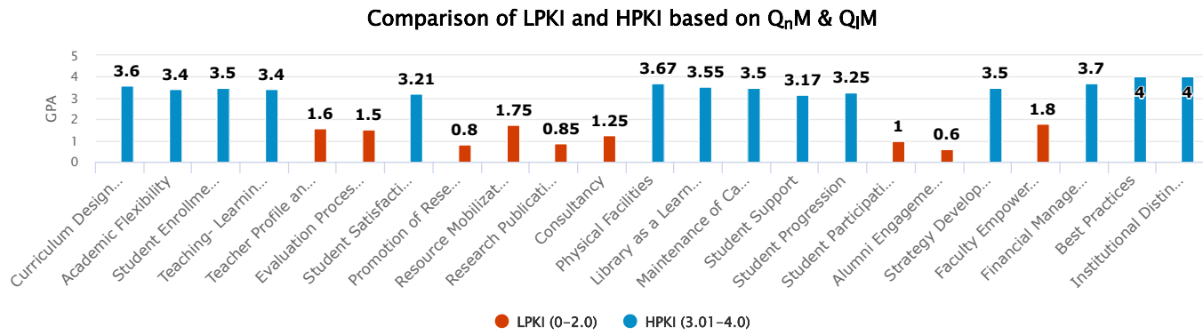
Fig: Comparison of LPKI(0-2.0) and HPKI(3.01-4.0) based on Q n M & Q m M
